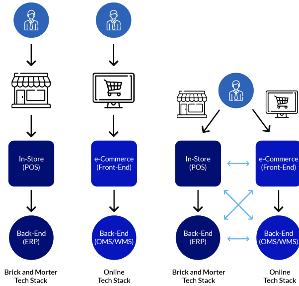
Figure 1: Traditional Models
