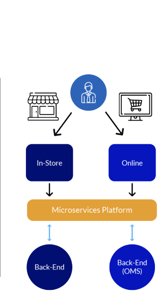
Figure 2: Aratum Approach
